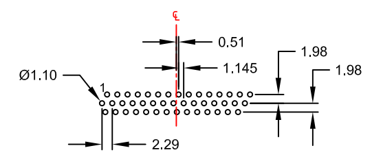
44-contact
